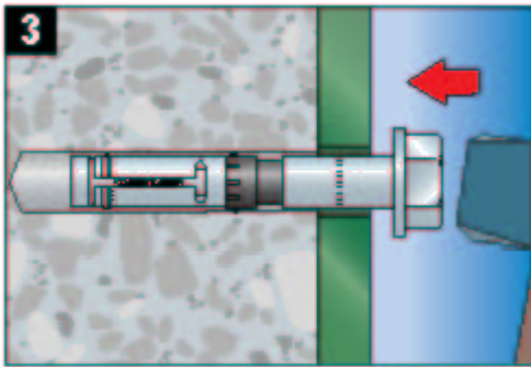
Install anchor
