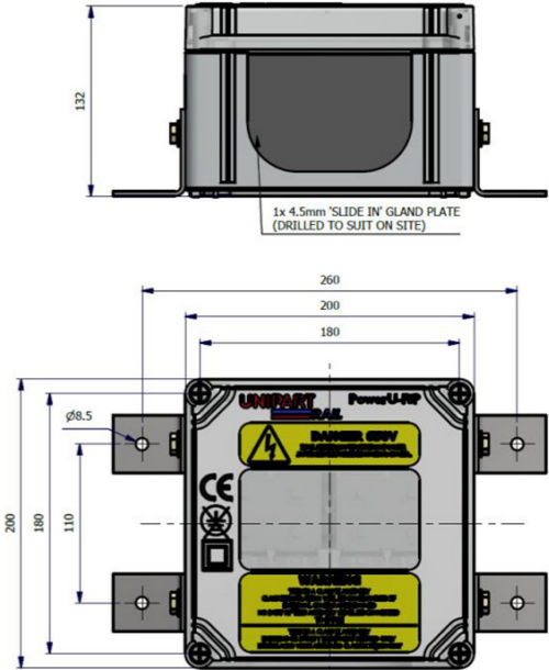
TBI & TB2 Overall dimensions
