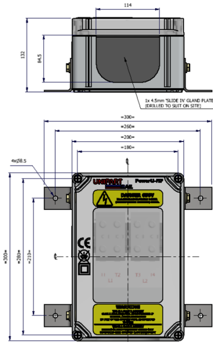
TB3 & TB4 Overall dimensions
